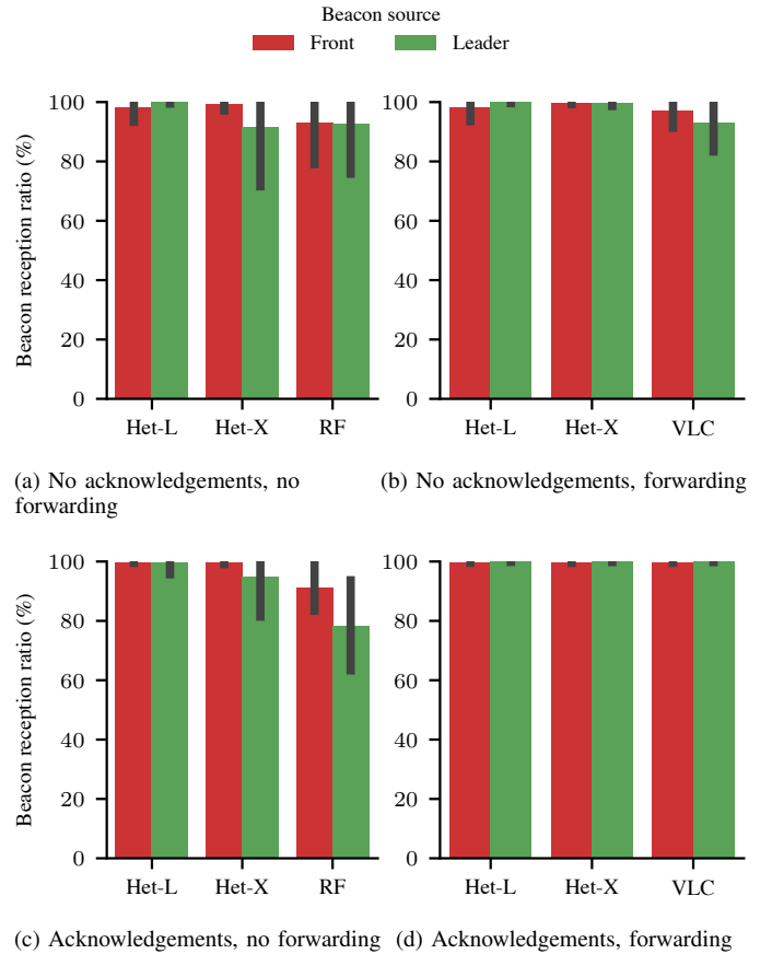
Figure 2. Beacon reception ratio with 160 vehicles. Data for disabled (first row) and enabled acknowledgements (second row) as well as disabled (first column) and enabled forwarding (second column) is shown. The mean of all simulation runs are shown, the error bar indicates the standard deviation. Note that data for RF and VLC is only available for dis- and enabled forwarding, respectively.
